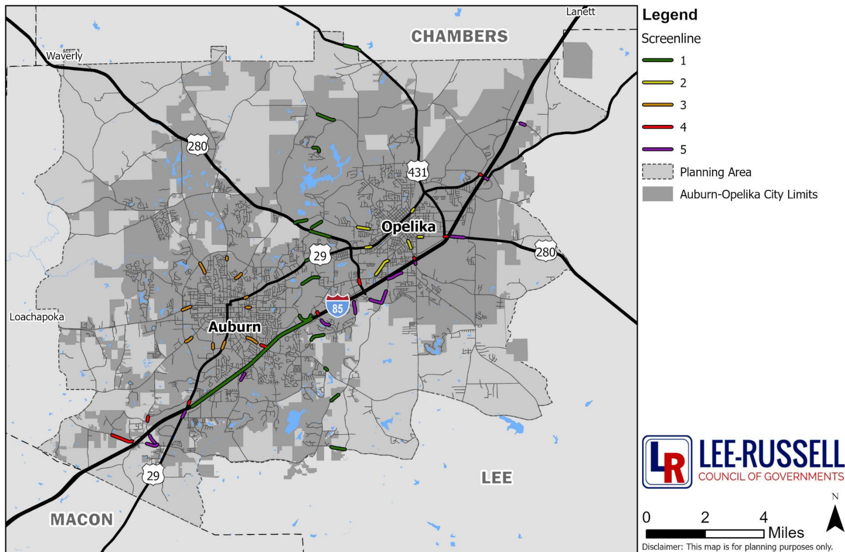
Figure 8.2: LRTP 2050 Screenlines
